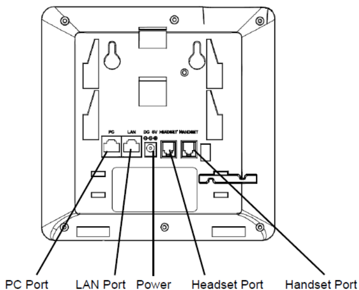
Figure 1: GXP1400/GXP1405 Ports
